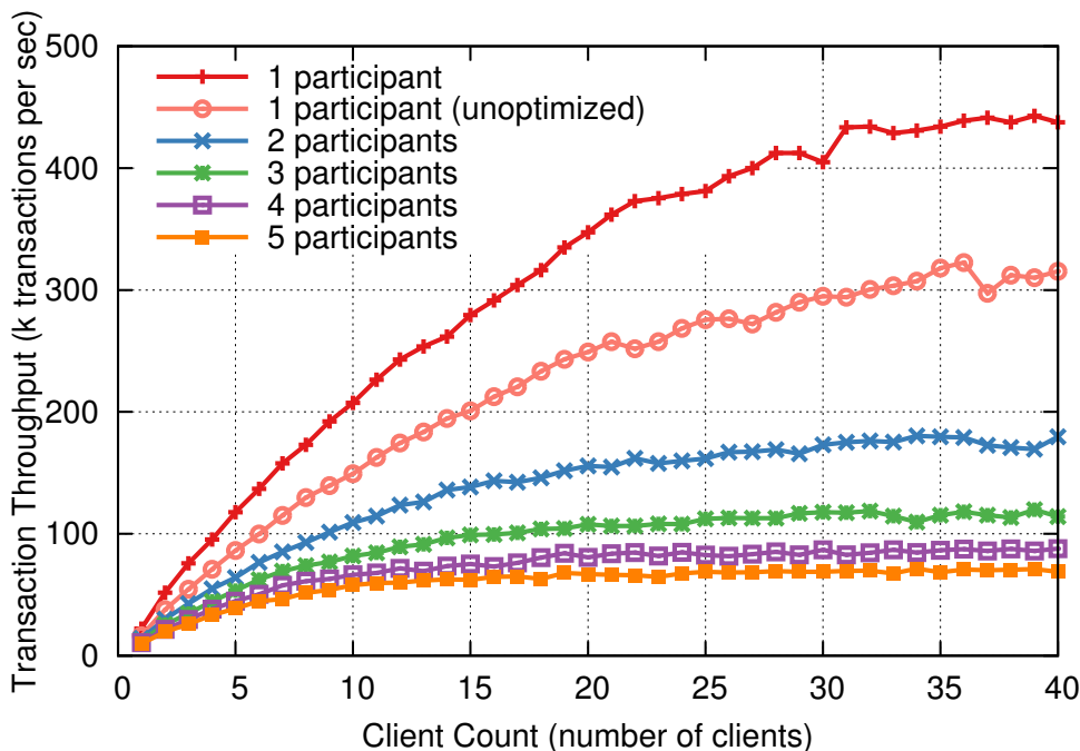
Figure 12: Aggregate transaction throughput for a cluster of 10 servers as a function of the number of clients. Each client repeatedly creates and commits transactions back to back where each transaction reads and writes one 100-byte object per participant; participants were chosen at random for each transaction. Each experiment was run 5 times; the figure shows the median measured throughput. The “unoptimized” case shows throughput with the single-server optimization disabled.
