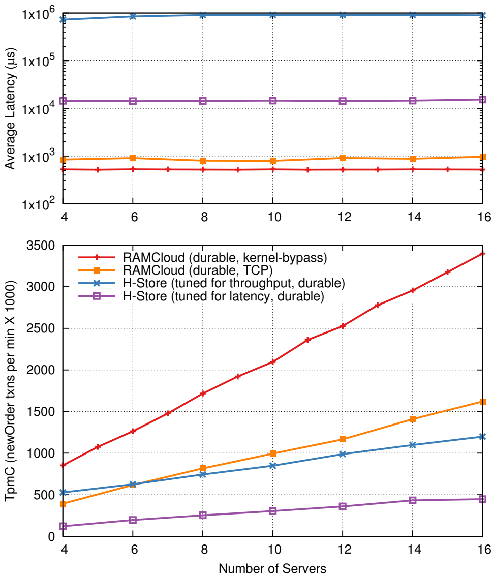
Figure 14: Latency and aggregate throughput of NewOrder transactions in the TPC-C benchmark, as a function of the system scale. The benchmark used the transaction mix in Table 2, with each warehouse stored on a single server. Increasing the number of servers also increased the number of warehouses. Roughly 90% of NewOrder transactions involved only one warehouse. RIFL-based transactions were tested on both RAMCloud’s standard kernel-bypassing Infiniband transport as well as kernel TCP.
