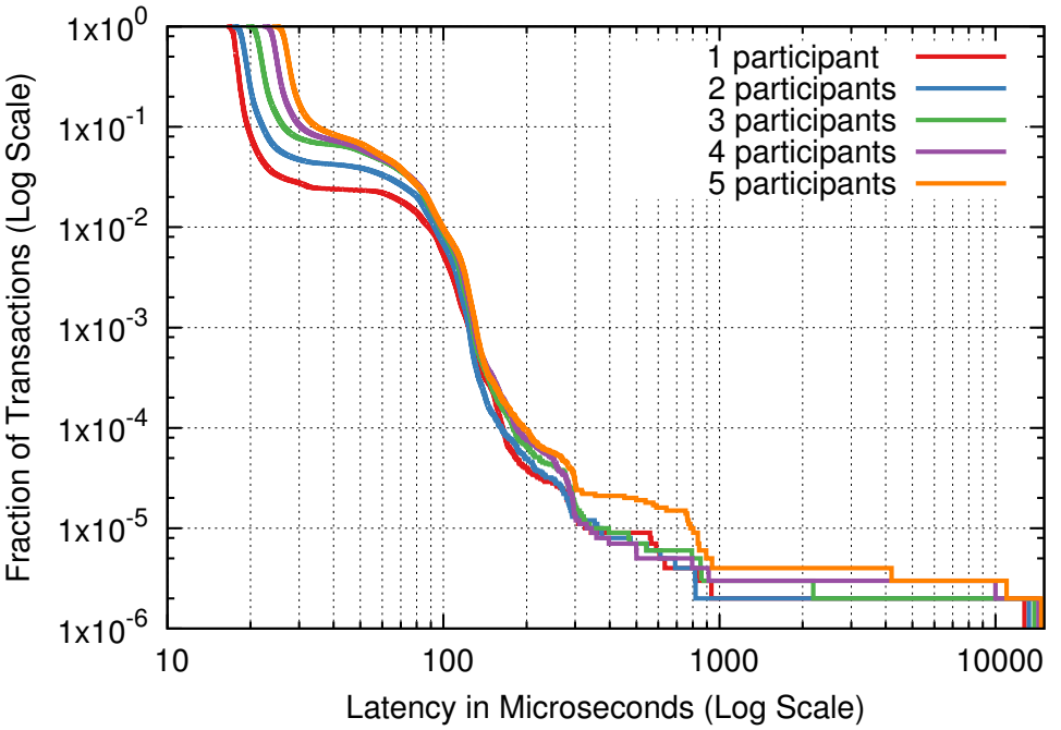
Figure 10: Reverse cumulative distribution of transaction commit latency measured from the beginning of the commit process to the completion of all prepare RPCs. Each transaction reads and writes one randomly chosen object per participant; the cluster contained 10 servers. A point (x, y) indicates that y of the 1M measured transaction commits took at least x \mu s to complete. The median latency for 1, 2, 3, 4, and 5 participants is 17.8 \mu s, 19.2 \mu s, 21.8 \mu s, 24.8 \mu s, and 27.3 \mu s respectively.
