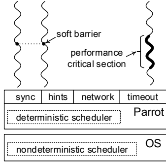
Figure 5: PARROT architecture.
