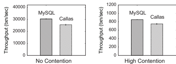
Fig. 11: Overhead of nexus locks
